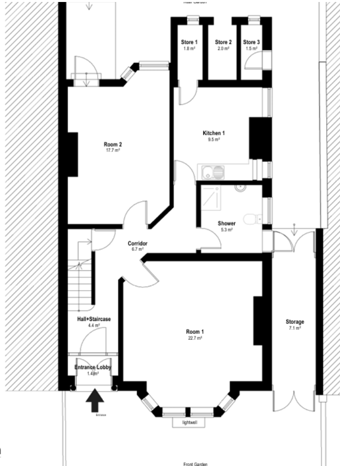
1 Existing Basement Floor Plan 1 : 50
