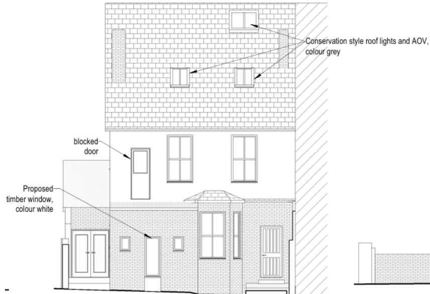
7 Proposed East Elevation 1 : 100
