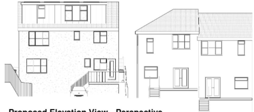
Proposed Elevation View - Perspective 1 : 100
