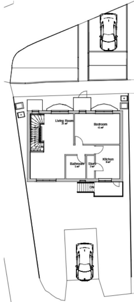
Proposed First Floor 1 : 100
